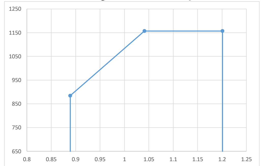
CBZ Weight & Balance Graph
